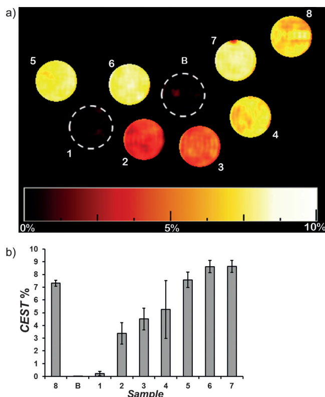
Figure 3. CEST images of phantoms at 37 °C on an MRI 4.7 T scanner with a pulse train comprised of five Gauss pulses at 12 \mu\text{T} for 1 s, interpulse delay of 200 \mu\text{s} at \pm 135 ppm. All solutions contain 40.0 mM HEPES buffer (pH 7.0), 200 mM NaCl, 8.0 mM \text{Co}^{\text{III}} / \text{Co}^{\text{II}} complex. a) 1) [\text{Co}(\text{TPT})]^{3+} ; 2) [\text{Co}(\text{TPT})]^{3+} and 0.25 equiv \text{Na}_2\text{S}_2\text{O}_4 ; 3) [\text{Co}(\text{TPT})]^{3+} and 0.38 equiv \text{Na}_2\text{S}_2\text{O}_4 ; 4) [\text{Co}(\text{TPT})]^{3+} and 0.50 equiv \text{Na}_2\text{S}_2\text{O}_4 ; 5) [\text{Co}(\text{TPT})]^{3+} and 0.75 equiv \text{Na}_2\text{S}_2\text{O}_4 ; 6) [\text{Co}(\text{TPT})]^{3+} and 1.0 equiv \text{Na}_2\text{S}_2\text{O}_4 ; 7) [\text{Co}(\text{TPT})]^{3+} and 1.25 equiv \text{Na}_2\text{S}_2\text{O}_4 ; 8) [\text{Co}(\text{TPT})]^{2+} . Scale represents the percent loss of signal because of CEST. b) Phantom image intensities (average of three experiments).
